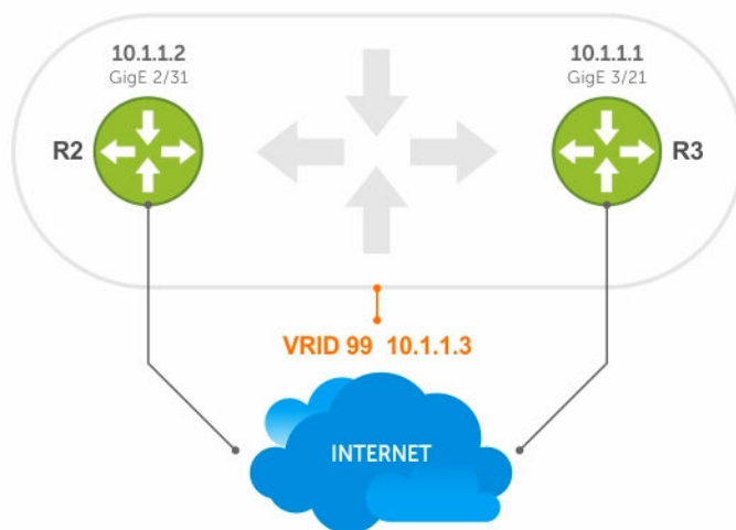
Figure 126. VRRP for IPv4 Topology
